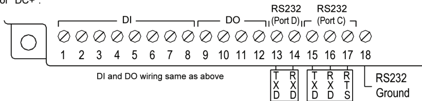
VT-UIPM-441 with 8 DI, 4 DO, 1 RS485 & 3 RS232
