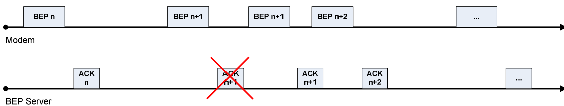
Figure 4: BEP Messages Acknowledgment with Retransmission
