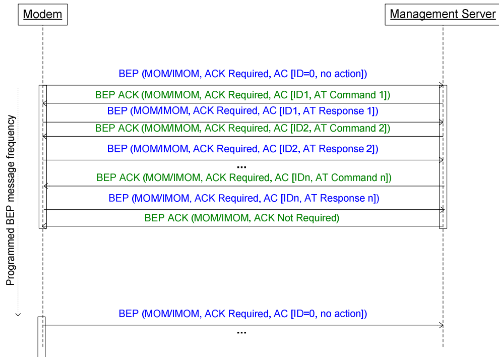
Figure 5: BEP/BEP ACK Messages Exchanges for MOM/IMOM
